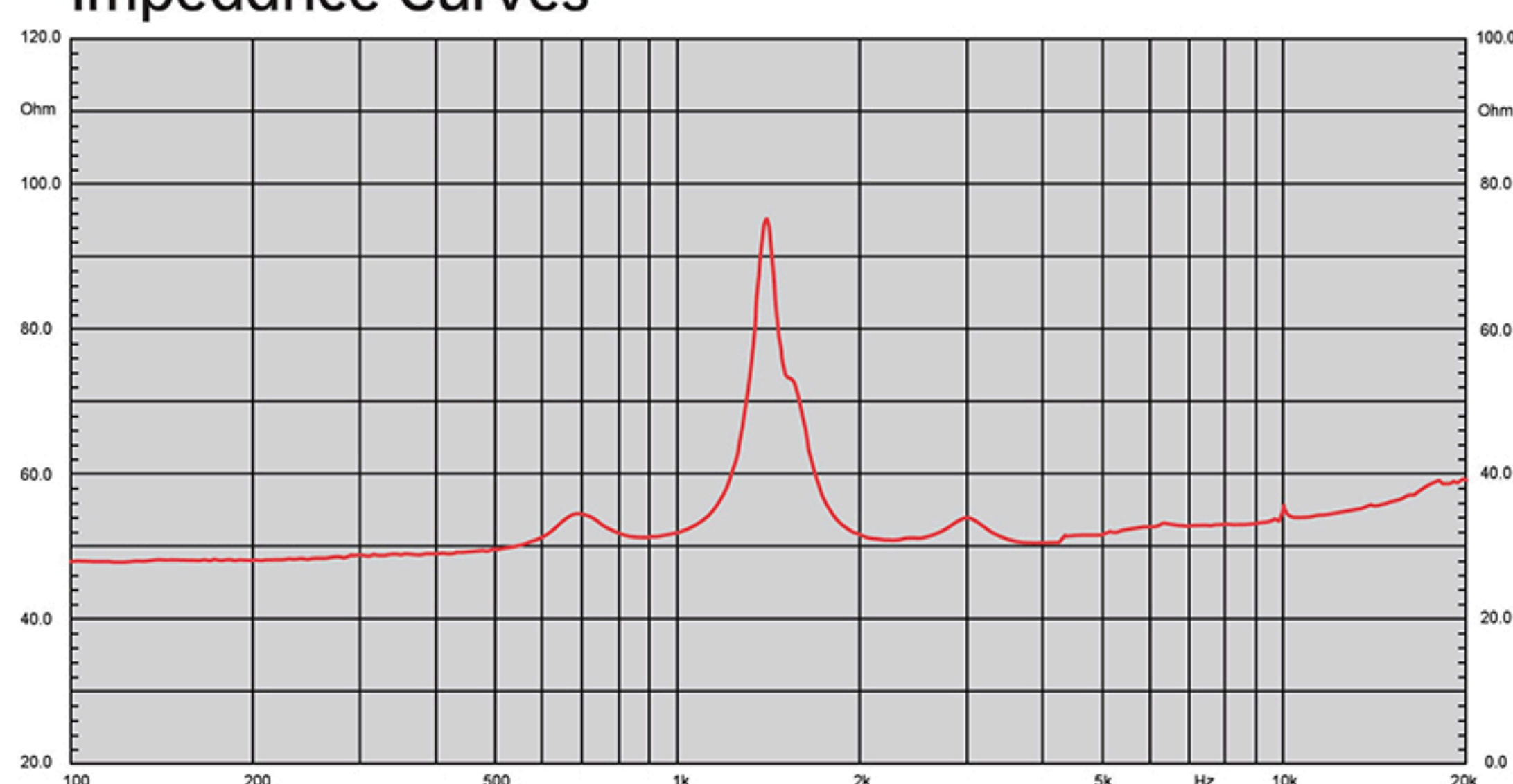
Impedance Curves
