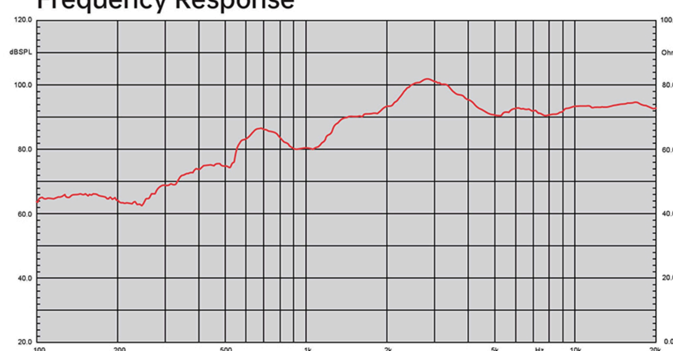
Frequency Response
