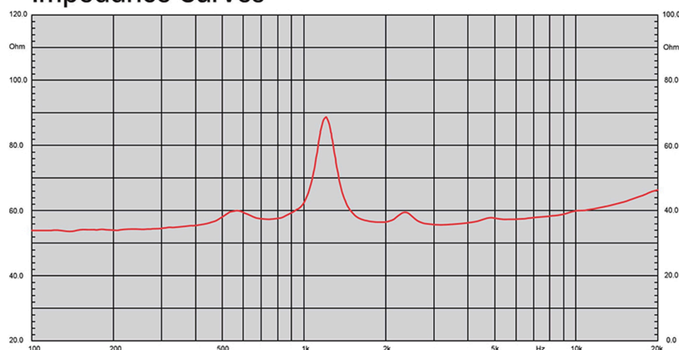
Impedance Curves
