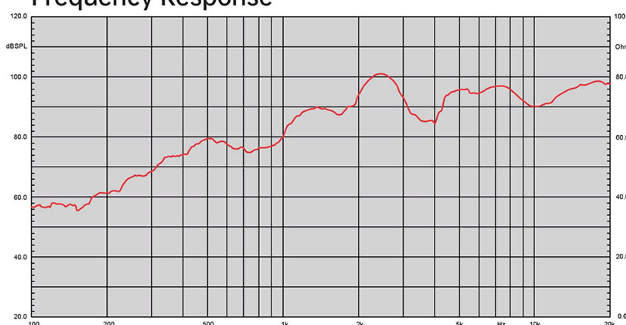
Frequency Response
